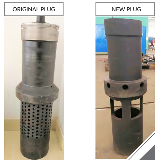
Redesigned plug assembly to resolve failure to open problem.
